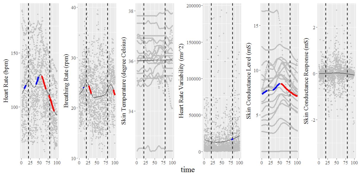
Fig. 4. SiZer analysis of the GMM predicted values after signal pre-processing treatment and feature extraction. A 99% point-wise confidence interval is shown. Significant periods are extracted from the first derivatives and reported on the actual GMM predicted values where red periods indicate a significant decrease and blue periods a significant increase. the period between the dashed black lines denotes the zipline activity.
